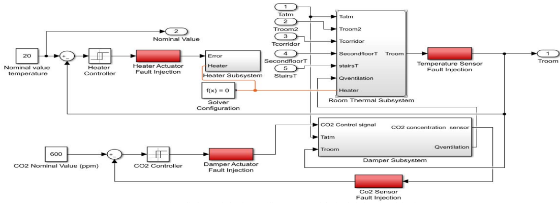
Fig. 4. Simulink model of an office room with fault injection blocks.
