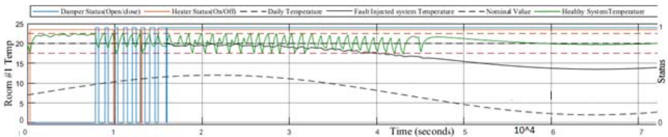
Fig. 8. The room number one temperature variation in healthy mode (green color) and faulty mode (black color) in case of activation CO 2 sensor fault.
